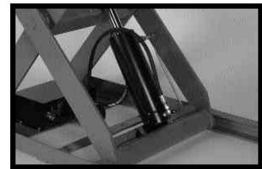
Quiet, efficient 1/2 HP bidirectional motor and pump assembly
